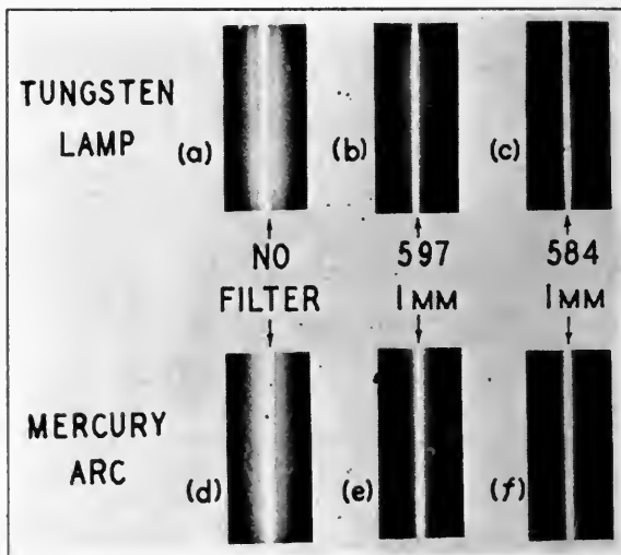
FIG. 7. Photographs of image structure for various conditions of exposure.
